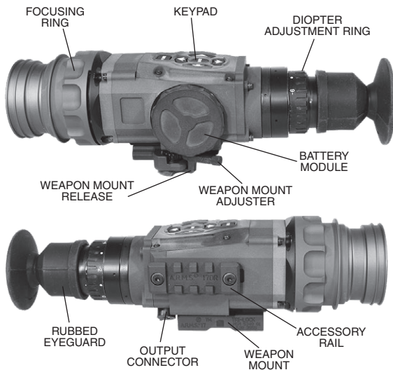
FIGURE 1.4. THOR MECHANICAL CONTROLS
