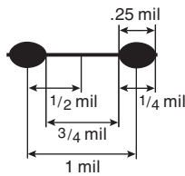
USMC Mil-dot Reticle
